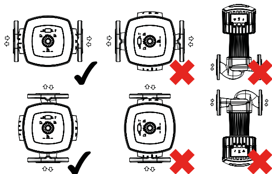
Fig. 6: Permissible installation positions Calio
