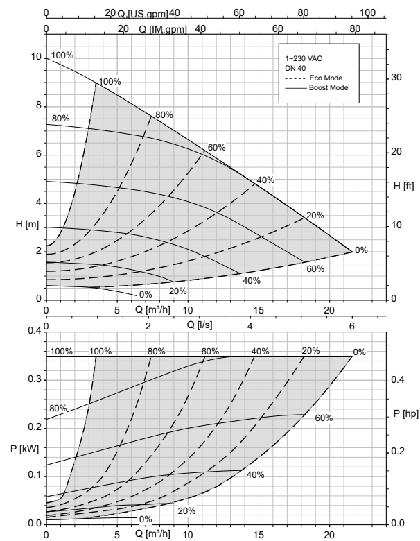
Calio 40-100 Open-loop Control, Eco Mode
