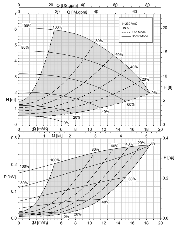
Calio 50-60 Open-loop Control, Eco Mode
