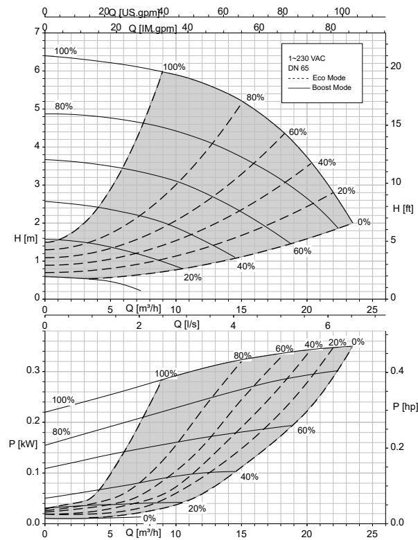
Calio 65-120 Open-loop Control, Eco Mode
