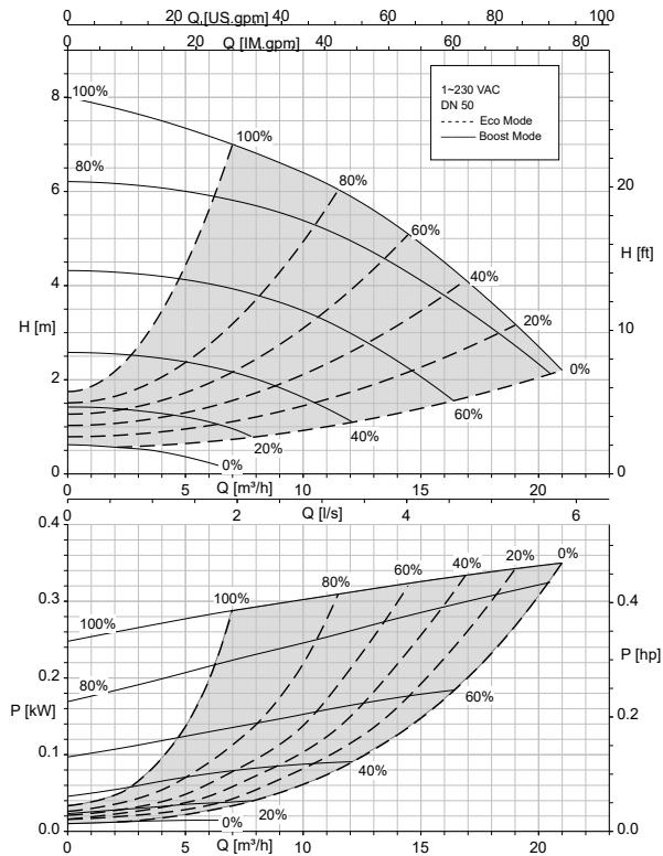
Calio 50-90 Open-loop Control, Eco Mode
