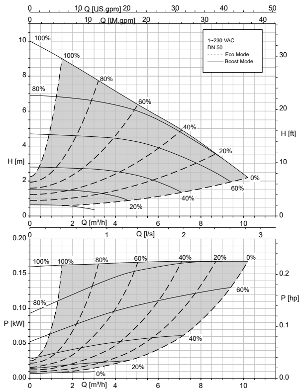
Calio 50-90 Open-loop Control, Eco Mode
